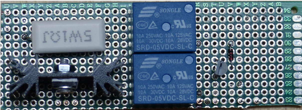
Bottom panel
