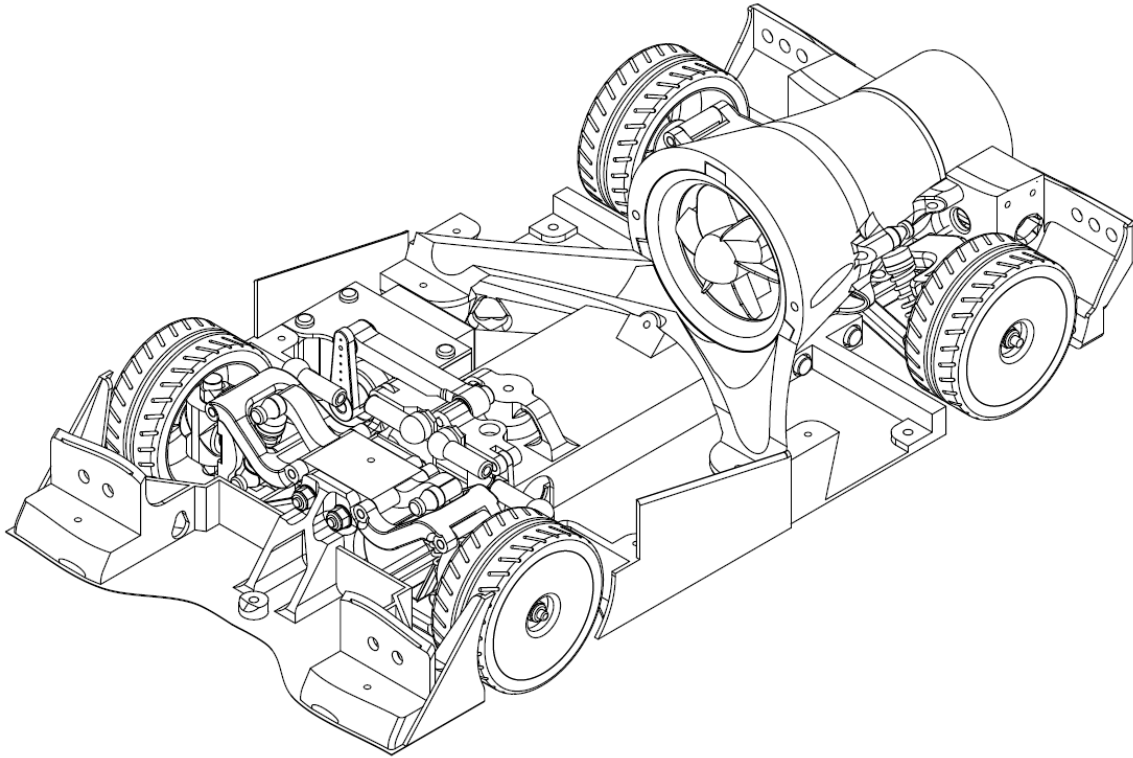
AS 03 Rear suspension Assembly
