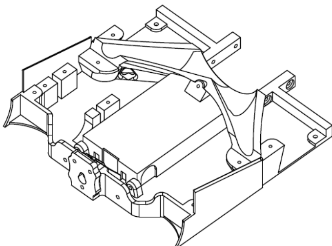
Part No 0001 Main Chassis
