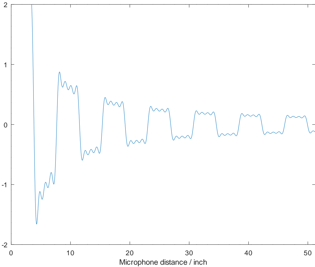
SWIMulator for first 4 Fourier terms of square wave
